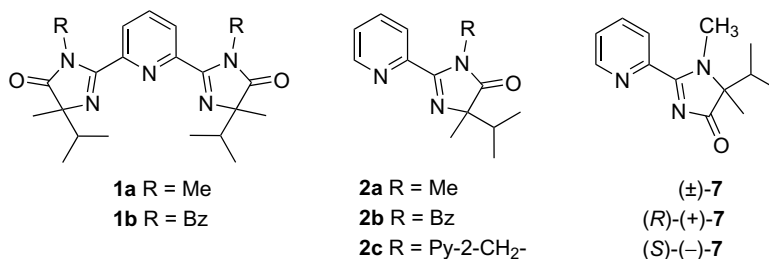
Chart 1. 4,5-Dihydro-1 H -imidazol-5(4)-one chiral ligands.
