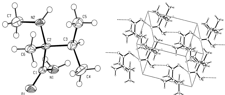
Figure 1. ORTEP representation and projection of crystal structure of compound ( R )-(+)-6.
