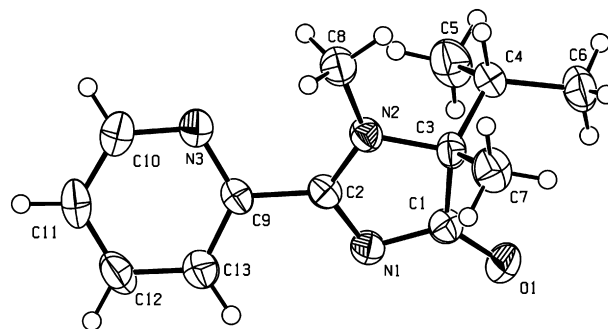
Figure 2. ORTEP representation of structure of compound ( R )-(+)-7.
